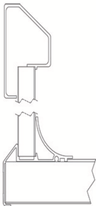
H.D. TOP AND BOTTOM RAIL PROFILE
